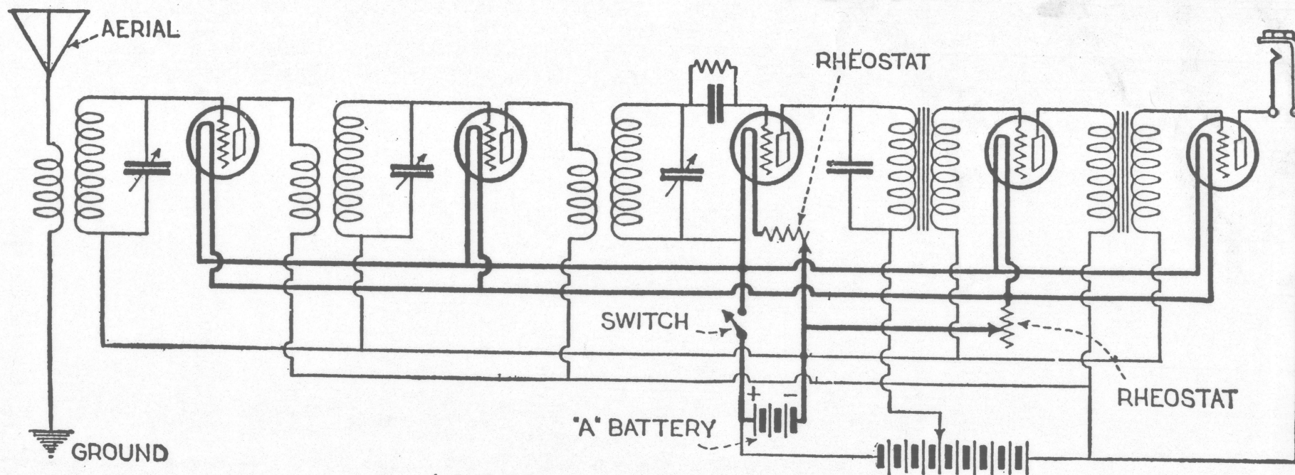
A standard five tube tuned radio frequency circuit.
