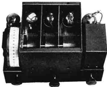
MODEL RECEIVER CHASSIS UTILIZING D. C. TETRODE
