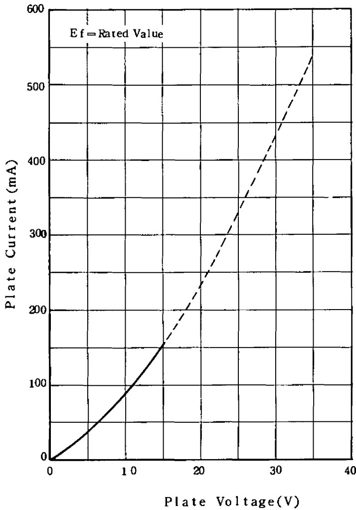
AVERAGE PLATE CHARACTERISTIC
