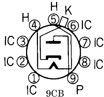
12BY3 BASING DIAGRAM: Bottom View
